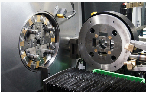
Example of the tools setup in the rotary swaging machine
