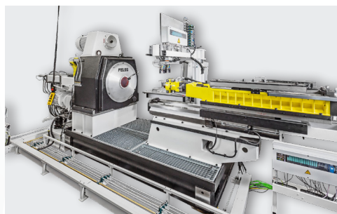
Single-station rotary swaging machine
